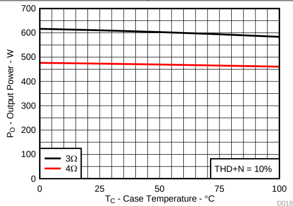
图 13. Output Power vs Case Temperature
