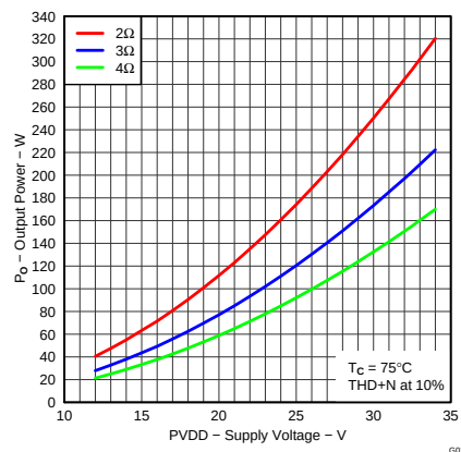
图 24. Output Power vs Supply Voltage
