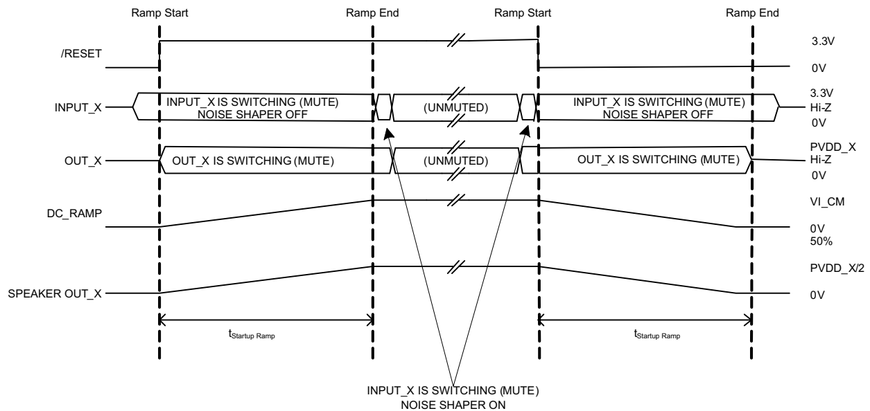
图 15. Start-up/Shutdown Ramp
