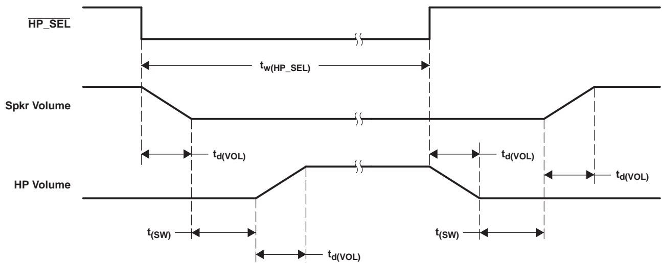
Figure 7. HP_SEL Timing
