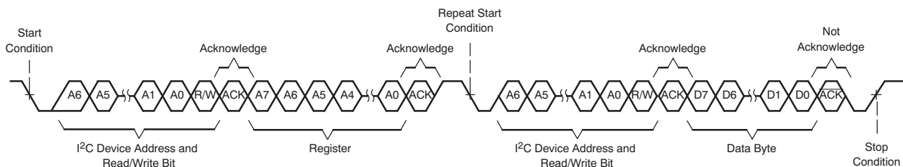
图 22. Single-Byte Read Transfer
