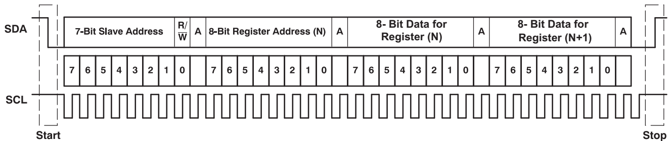
图 19. Typical I²C Sequence
