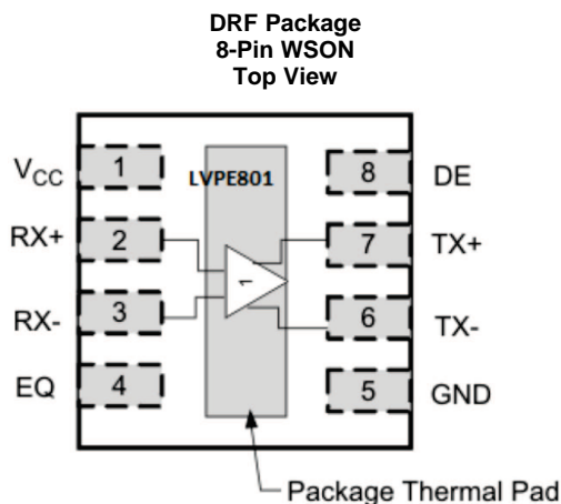
Pin Functions
