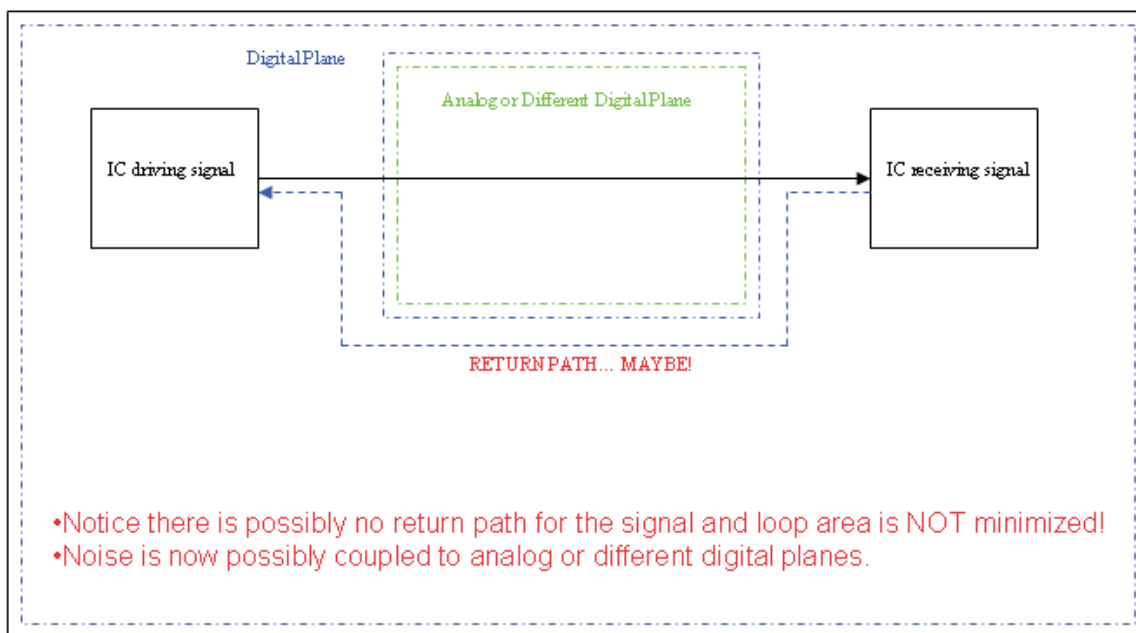
Figure 29. Incorrect Routing
