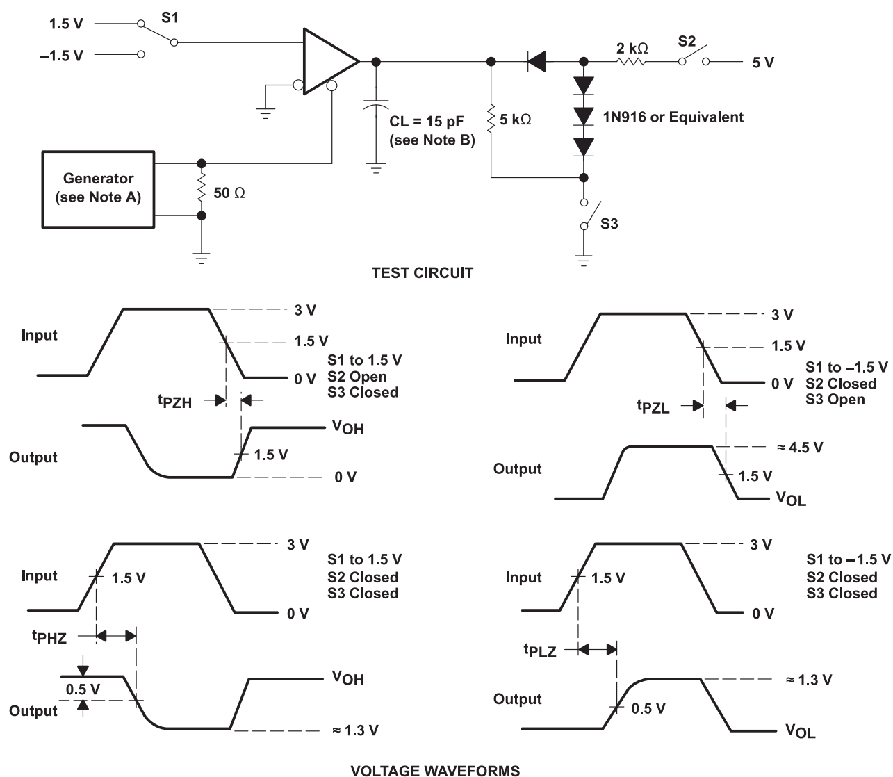
图 7-6. Receiver Test Circuit and Voltage Waveforms
