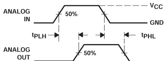
图 6-7. Propagation Delays, Analog in to Analog Out
