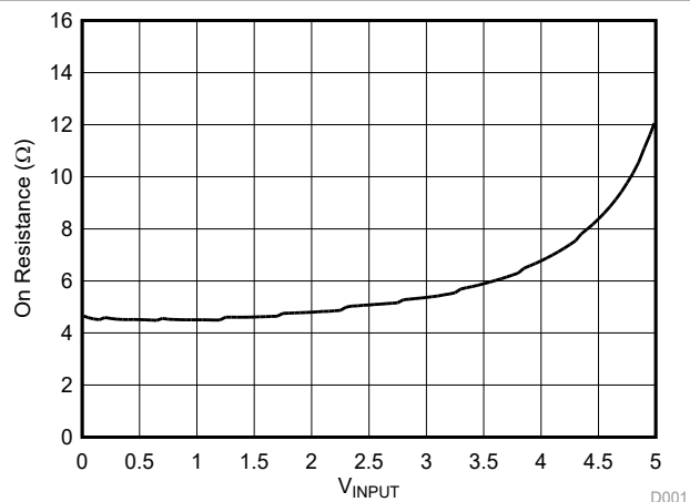
图 4-1. Log r_{on} 与 V_I 间的关系, V_{CC} = 3.3V 且 I_O = -15mA
