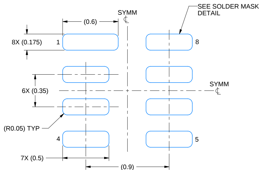
LAND PATTERN EXAMPLE EXPOSED METAL SHOWN SCALE: 40X
