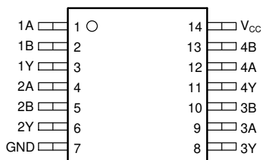
图 5-1. SN54AHCT86 J or W Package, 14-Pin (Top View)
