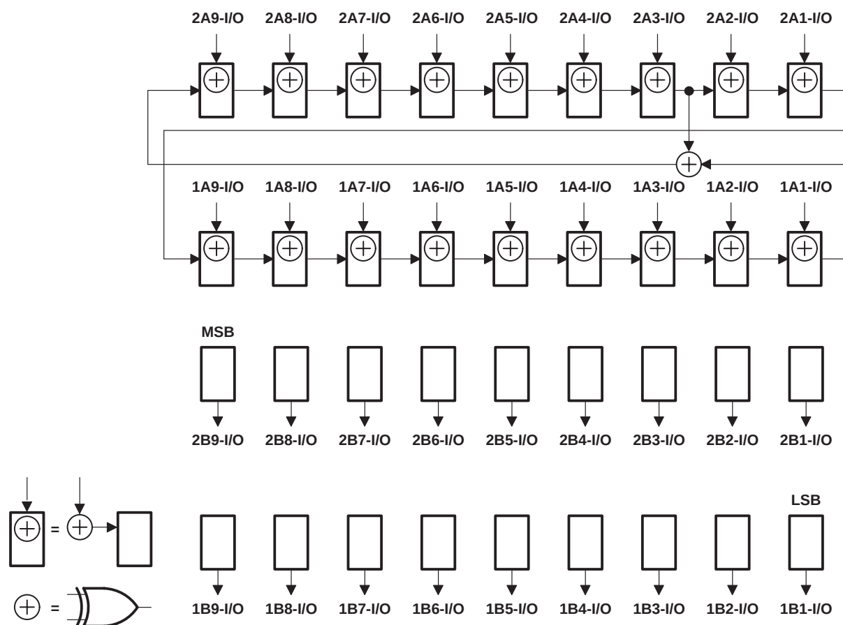
Figure 11. 18-Bit PSA/COUNT Configuration (1OEA = 2OEA = 0, 1OEB = 2OEB = 1)
