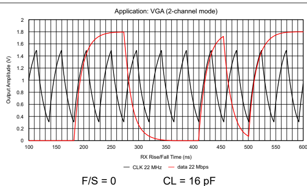
The data signal has a slower maximum switching frequency, and therefore drives a larger amplitude than the clock signal. 图 9-4. Output Amplitude vs Toggling Frequency (F/S = 0)
