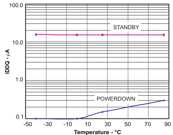
图 6-2. Quiescent Supply Current vs Temperature
