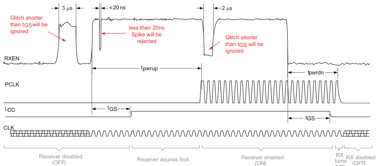
图 7-10. Receiver Enable and Disable Glitch Suppression Time
