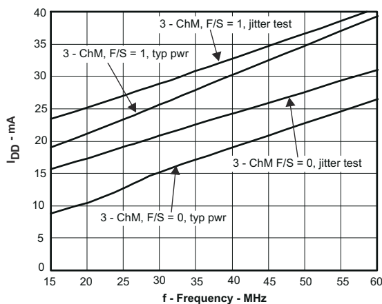
图 6-5. Supply Current vs Frequency, 3-Channel Mode
