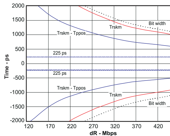
图 6-10. RSKM, 2-Channel Mode vs Bit Rate
