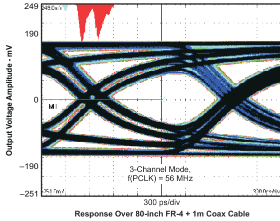
图 6-12. XGA 3-Channel Output Waveform
