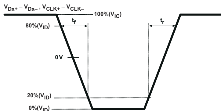
图 7-4. SubLVDS Differential Input Rise and Fall Time Defintion
