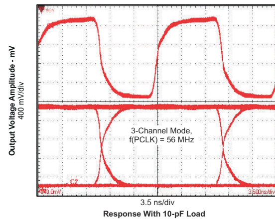
图 6-13. XGA 3-Channel Output Waveform
