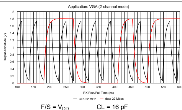
图 9-3. Output Amplitude vs Toggling Frequency (F/S = 1)
