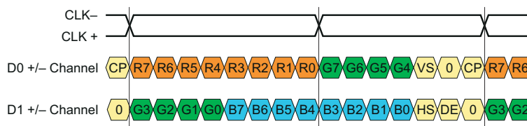
图 8-5. Data and Clock Output in 2-Channel Mode (LS0 = high; LS1 = low).
