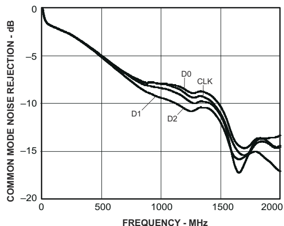
图 6-20. Output Common Mode Noise Rejection
