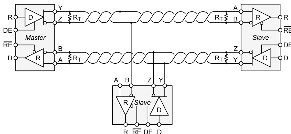
图 10-2. Typical RS-485 Network With Full-duplex Transceivers
