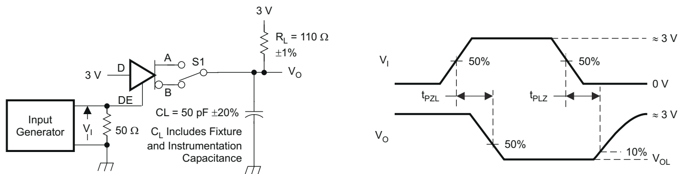
图 8-5. Measurement of Driver Enable and Disable Times With Active-Low Output and Pullup Load
