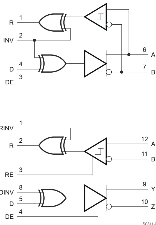
图 9-5. SN65HVD17xx Options With Inverting Feature to Correct for Miswired Cables
