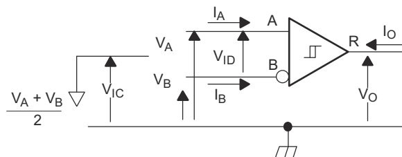
图 8-8. Receiver Voltage and Current Definitions
