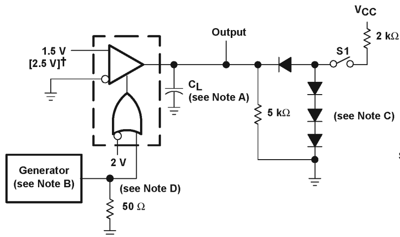
图 6-1. t_{PLH} , T_{PHL} Test Circuit and Voltage Waveforms
