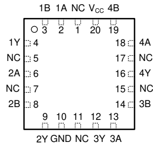
图 5-3. SN54AHCT86 FK Package, 20-Pin (Top View)
