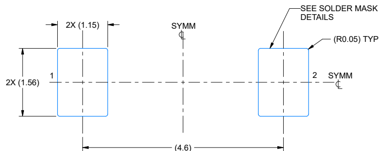
LAND PATTERN EXAMPLE EXPOSED METAL SHOWN SCALE 15X
