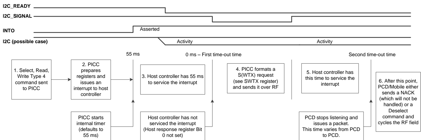
图 5-17. Timing Limits
