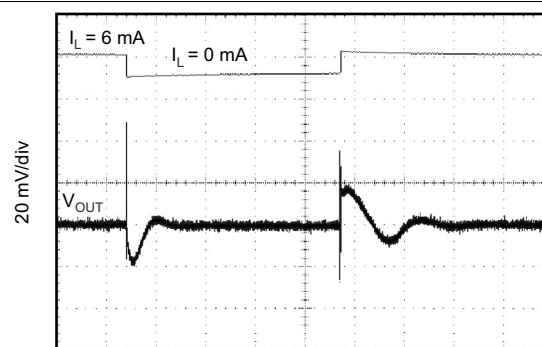
40 \mu\text{s}/\text{div} C_L = 1\text{ }\mu\text{F} 图 6-47. 1mA 至 6mA 负载瞬态
