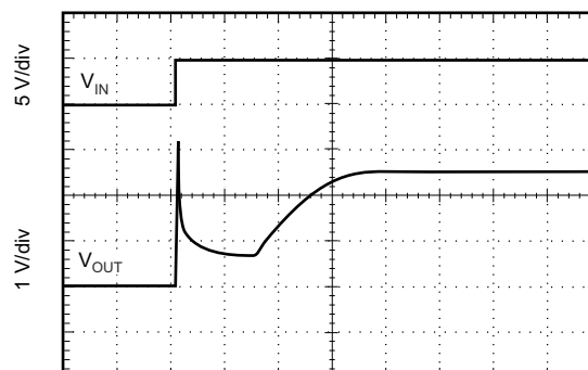
10 \mu\text{s}/\text{div} C_L = 0 , 5V 启动
