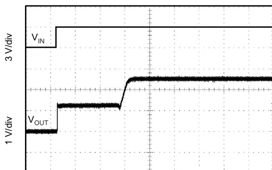
40 \mu\text{s}/\text{div} C_L = 0 , 3V 启动
