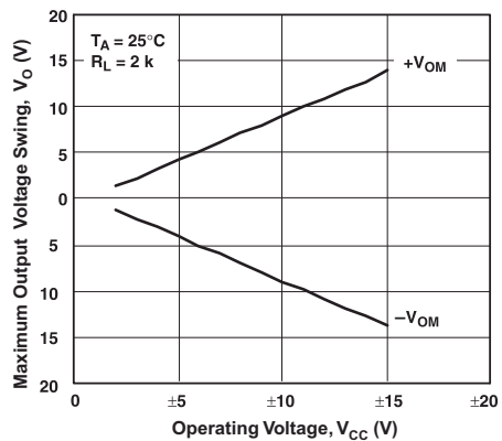
图 5-9. Maximum Output Voltage Swing vs Operating Voltage
