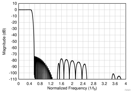
图 7-25. Linear Phase Decimation Filter Magnitude Response
