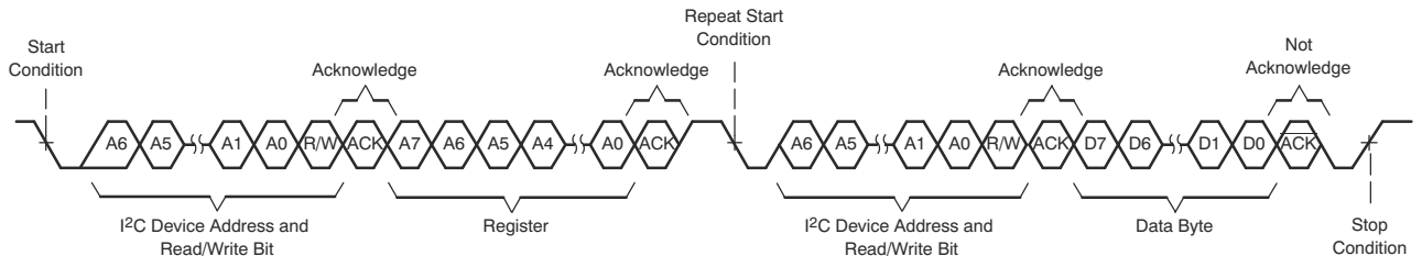
图 7-66. I 2 C Single-Byte Read Transfer
