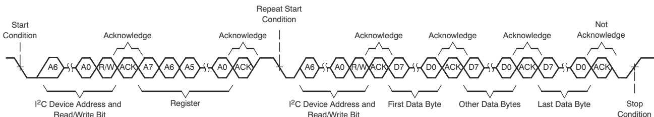
图 7-67. I 2 C Multiple-Byte Read Transfer
