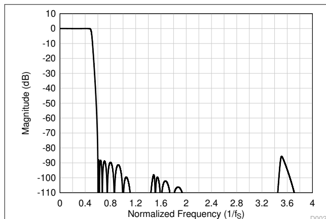
图 7-47. Low-Latency Decimation Filter Magnitude Response
