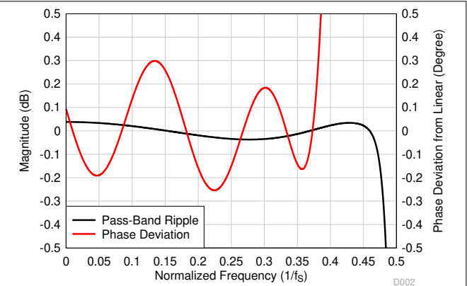
图 7-46. Low-Latency Decimation Filter Pass-Band Ripple and Phase Deviation
