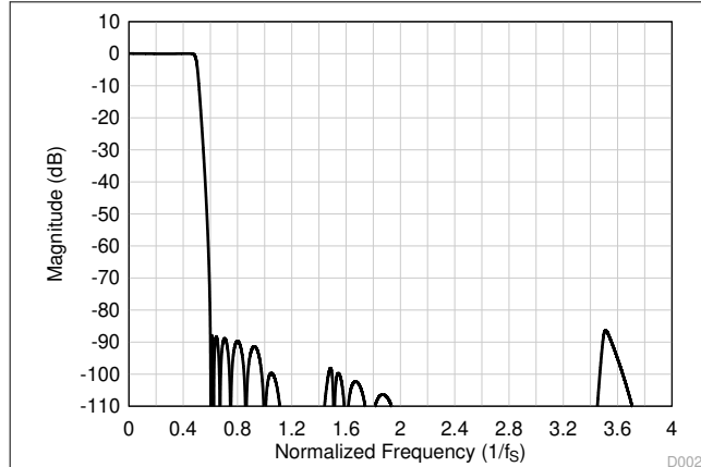
图 7-45. Low-Latency Decimation Filter Magnitude Response
