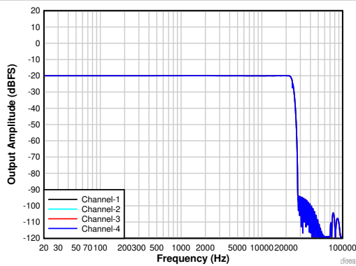
5th-order PDM modulator with \text{PDMCLKx} = 3.072\text{ MHz}
