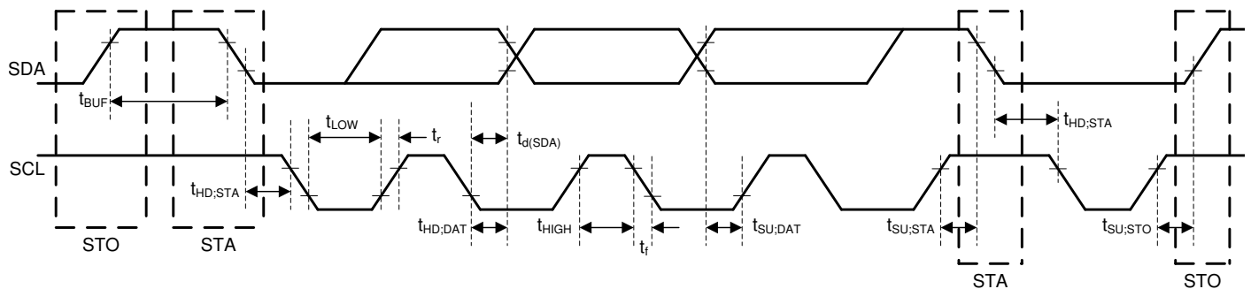
图 6-1. I²C Interface Timing Diagram
