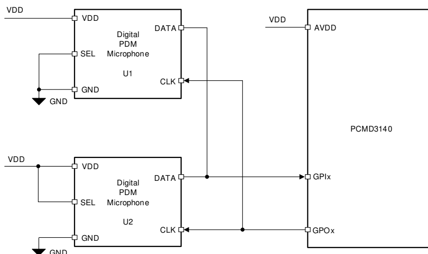
图 7-14. Digital PDM Microphones Connection Diagram to the PCMD3140
