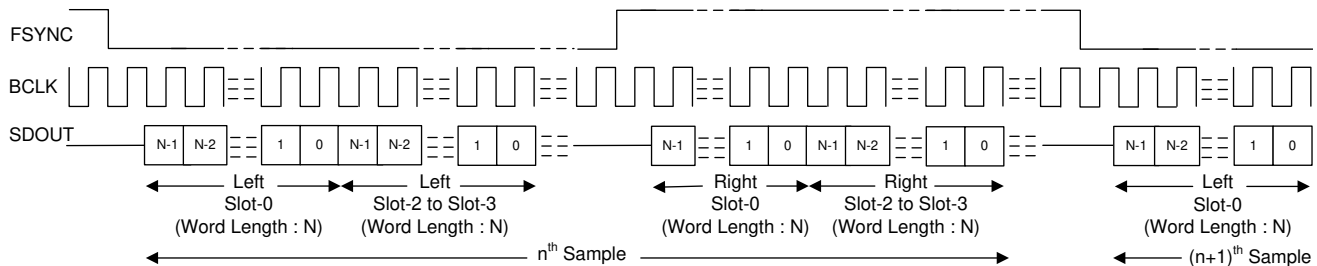
图 7-5. I²S Mode Standard Protocol Timing (TX_OFFSET = 0)
