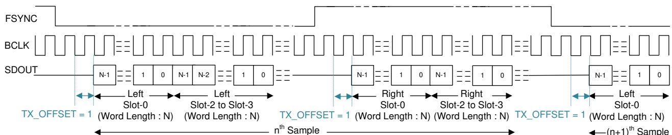
图 7-6. I²S Protocol Timing (TX_OFFSET = 1)
