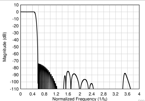
图 7-27. Linear Phase Decimation Filter Magnitude Response
