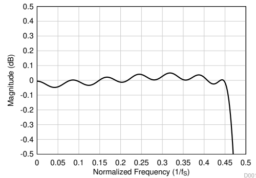
图 7-22. Linear Phase Decimation Filter Pass-Band Ripple
