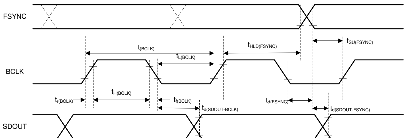
图 6-2. TDM (With BCLK_POL = 1), I²S, and LJ Interface Timing Diagram
