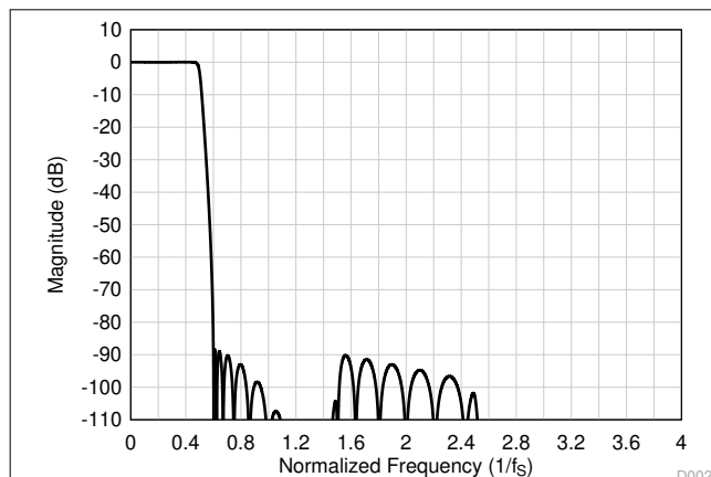
图 7-41. Low-Latency Decimation Filter Magnitude Response
