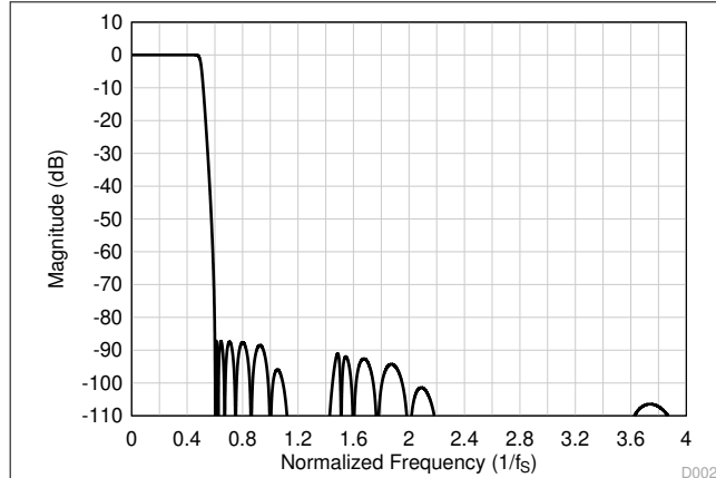
图 7-39. Low-Latency Decimation Filter Magnitude Response
