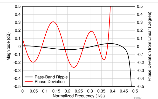
图 7-42. Low-Latency Decimation Filter Pass-Band Ripple and Phase Deviation
