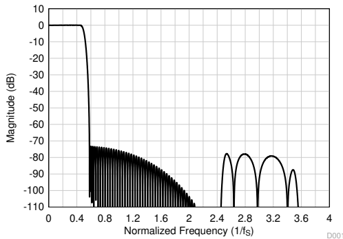
图 7-21. Linear Phase Decimation Filter Magnitude Response
