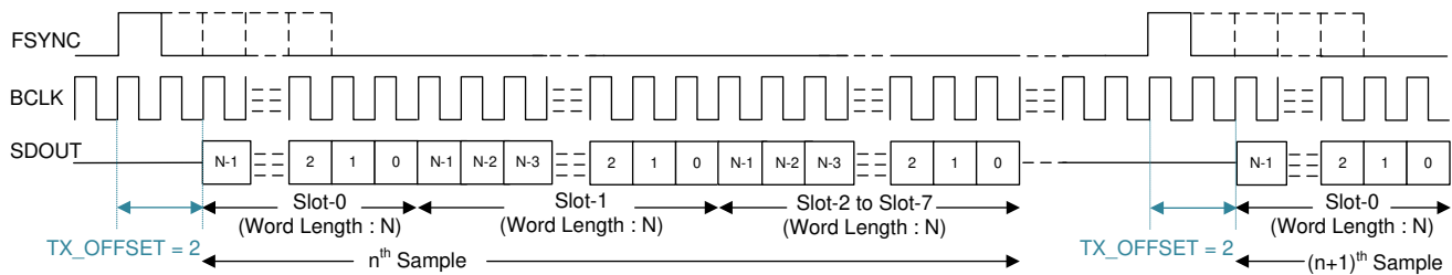
图 7-2. TDM Mode Protocol Timing (TX_OFFSET = 2)
