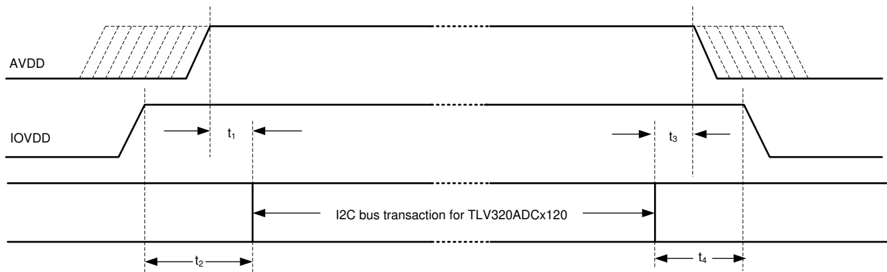
图 9-1. Power-Supply Sequencing Requirement Timing Diagram
