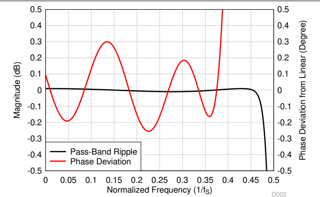
图 7-40. Low-Latency Decimation Filter Pass-Band Ripple and Phase Deviation
