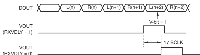
图 7-15. RXVDLY and VOUT Timing
