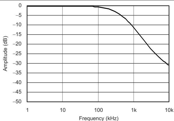
图 6-8. Antialiasing Filter Characteristic
