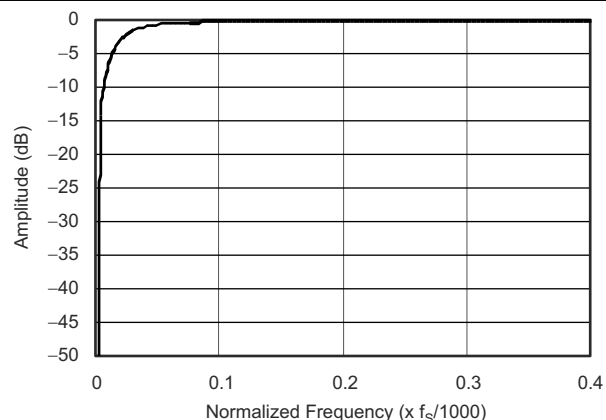
图 6-7. High-Pass Filter Characteristic
