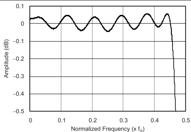
图 6-6. Decimation Filter Passband Characteristic
