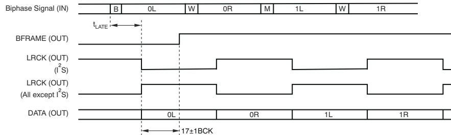
图 7-12. Latency Time Between Input Biphase and LRCKO/DOUT
