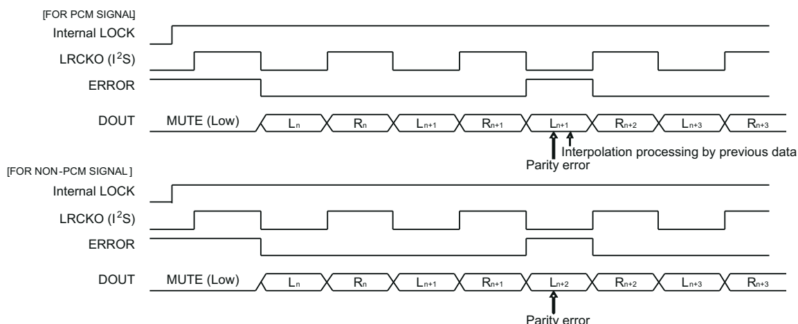
图 7-16. Processing for Parity Error Occurrence
