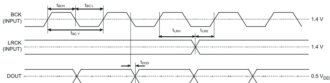
图 7-5. Audio Data Interface Timing (Slave Mode: BCK and LRCK Work as Inputs)
