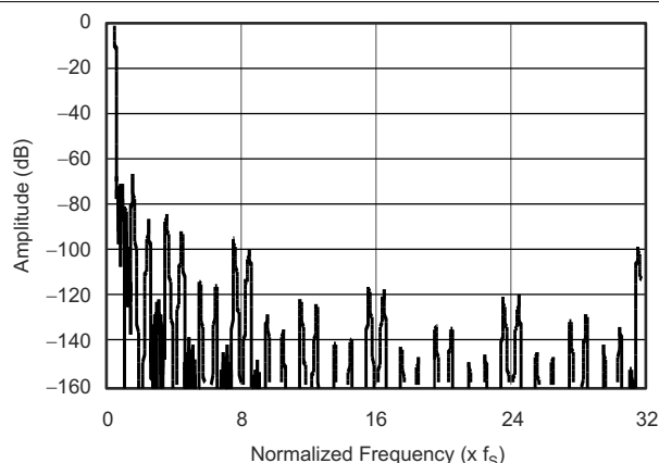
图 6-5. Decimation Filter Stop Band Characteristic
