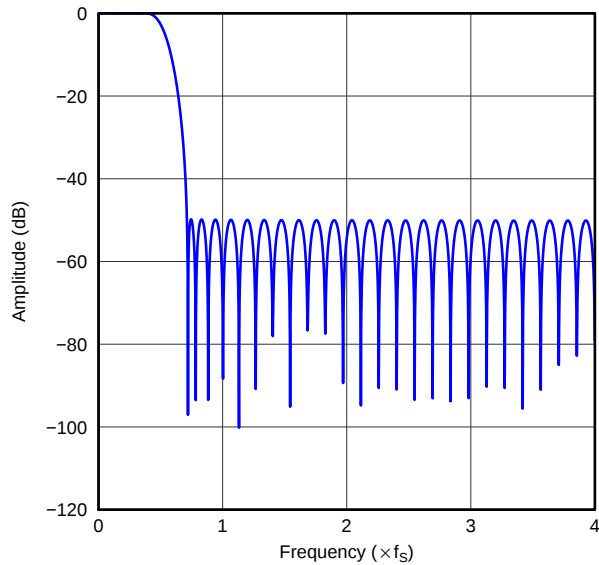
Figure 39. Asymmetric FIR x8 Interpolation Filter Frequency Response, Single Rate
