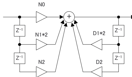
Figure 59. Biquad Block
