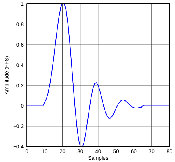
Figure 40. Asymmetric FIR x8 Interpolation Filter Impulse Response, Single Rate
