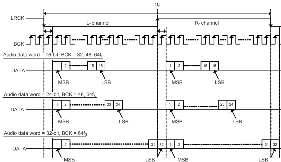
Figure 14. I²S Audio Data Format
