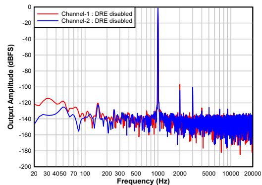
图 7-12. Differential Input: FFT With a -1\text{-dBr} Input
