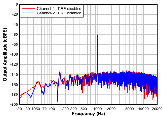
图 7-11. Differential Input: FFT With a -60\text{-dBr} Input and DRE Disabled
