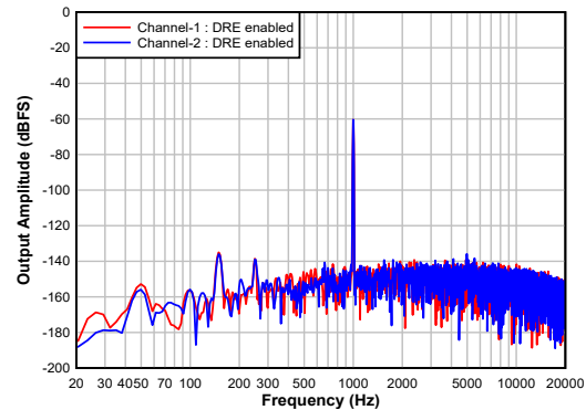
图 7-10. Differential Input: FFT With a -60\text{-dBr} Input and DRE Enabled
