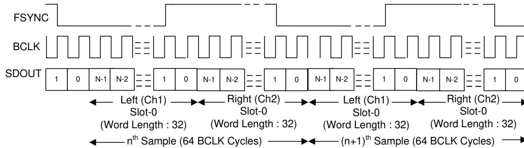
图 8-6. I²S Protocol Timing in Master Mode
