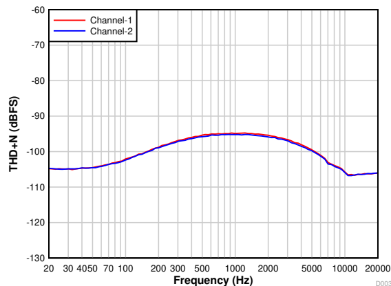
图 7-15. PCM1821-Q1: THD+N vs Input Frequency With a -1-dBr Input
