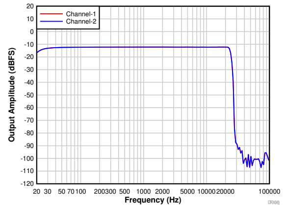
图 7-6. PCM1820-Q1: Frequency Response With a -12-dBr Input
