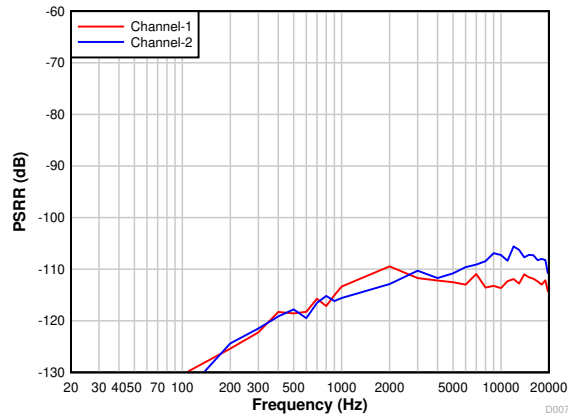
图 7-7. PCM1820-Q1: Power-Supply Rejection Ratio vs Ripple Frequency With a 100-mV pp Amplitude
