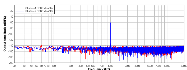
图 9-4. PCM1820-Q1: FFT With a - 60-dBr Input With DRE Disabled
