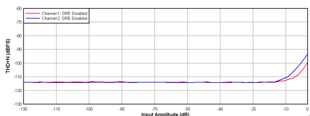
图 9-5. PCM1820-Q1: THD+N vs Input Amplitude With DRE Disabled
