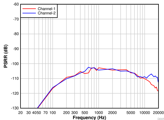
图 7-17. PCM1821-Q1: Power-Supply Rejection Ratio with Ripple Frequency With a 100-mV PP Amplitude
