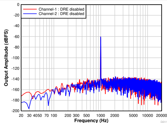
图 7-11. PCM1820-Q1: FFT With a -60-dBr Input and DRE Disabled
