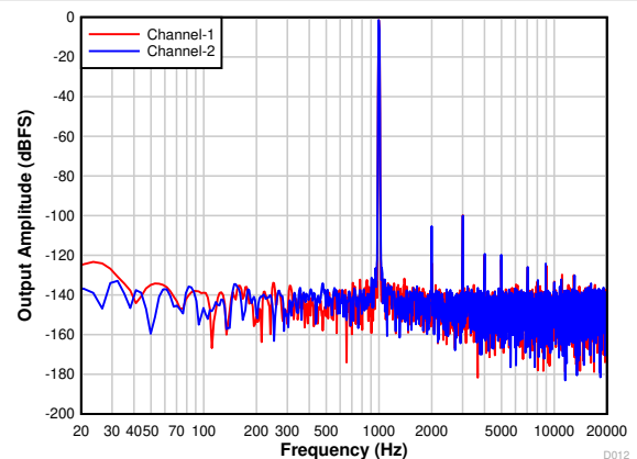
图 7-12. PCM1820-Q1: FFT With a -1-dBr Input
