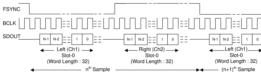
图 8-5. I²S Mode Protocol Timing in Slave Mode
