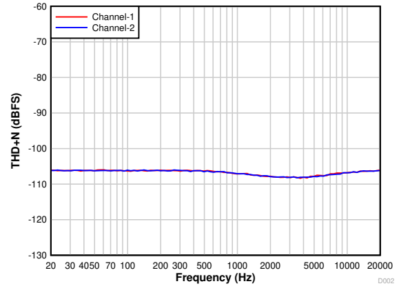
图 7-14. PCM1821-Q1: THD+N vs Input Frequency With a -60-dBr Input
