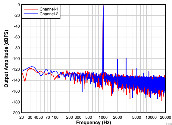
图 7-20. PCM1821-Q1: FFT With a -1-dBr Input
