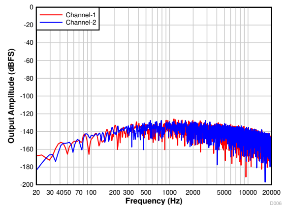
图 7-18. PCM1821-Q1: FFT With Idle Input and DRE Disabled
