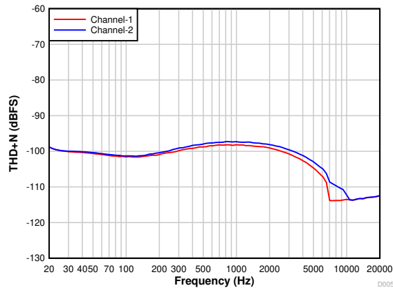
图 7-5. PCM1820-Q1: THD+N vs Input Frequency With a -1-dBr Input
