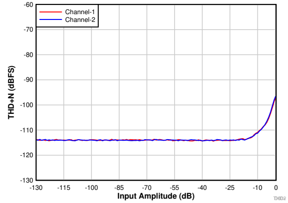
图 7-2. PCM1820-Q1: THD+N vs Input Amplitude With DRE Disabled
