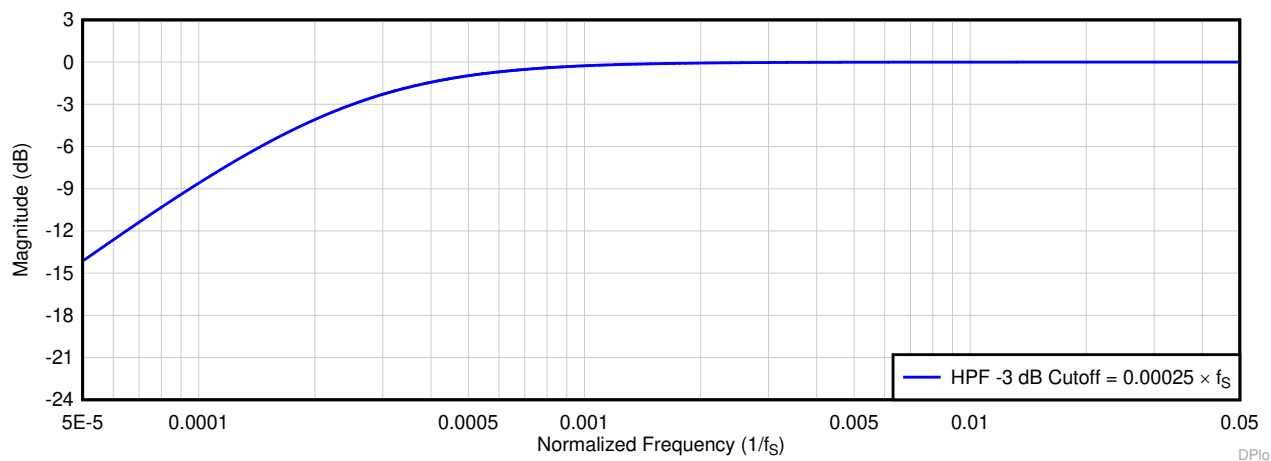
图 8-8. HPF Filter Frequency Response Plot
