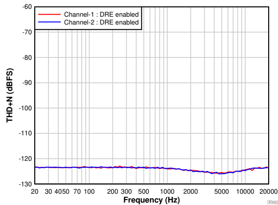
图 7-3. PCM1820-Q1: THD+N vs Input Frequency With a -60-dBr Input
