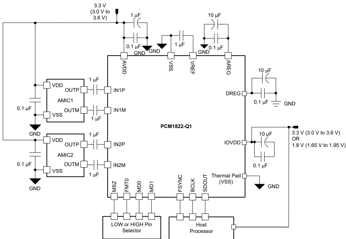
图 9-1. Two-Channel Analog Microphone Recording Diagram for 3.3-V AVDD Operation
