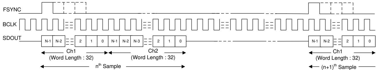
图 8-2. TDM Mode Protocol Timing (FMT0 = HIGH) In Slave Mode
