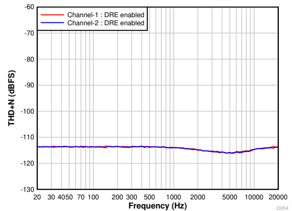
图 7-4. PCM1820-Q1: THD+N vs Input Frequency With a -60-dBr Input
