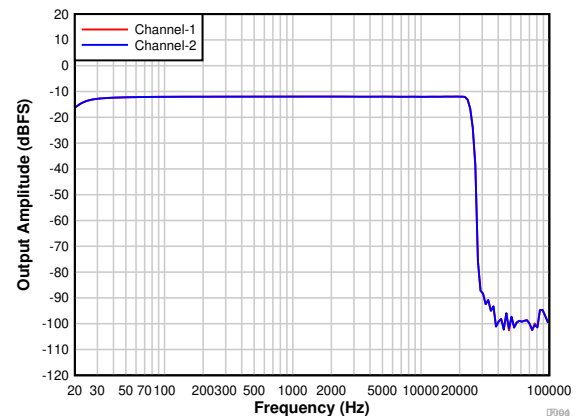
图 7-16. PCM1821-Q1: Frequency Response With a -12-dBr Input
