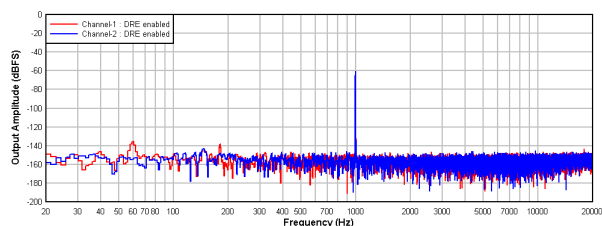
图 9-2. PCM1820-Q1: FFT With a - 60-dBr Input With DRE Enabled
