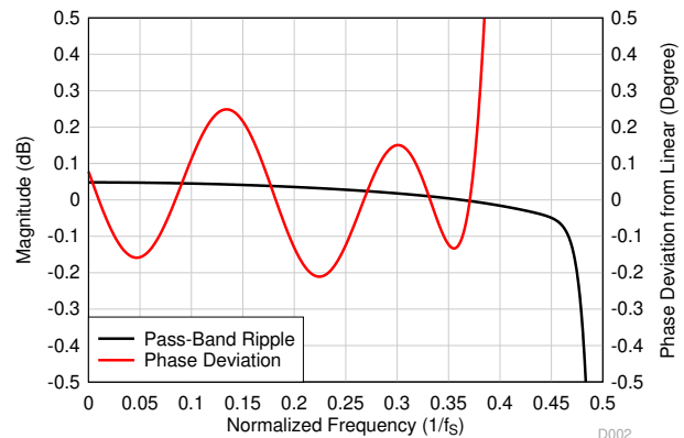
图 8-22. Low-Latency Decimation Filter Pass-Band Ripple and Phase Deviation
