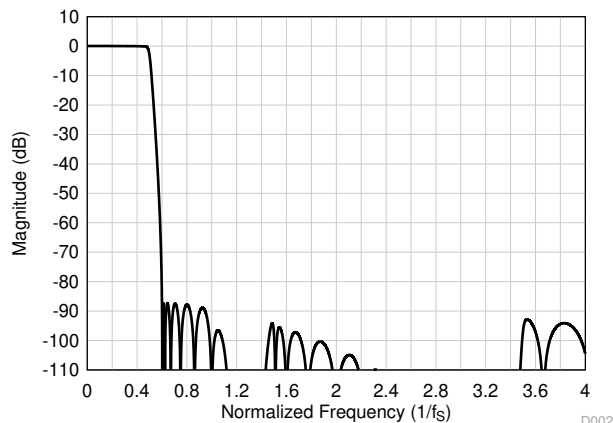
图 8-21. Low-Latency Decimation Filter Magnitude Response
