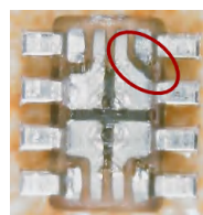
图 9-8. Identifying Package Orientation - Backside
