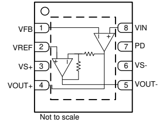
图 5-2. DTK Package, 8-Pin WSON (Top View)
