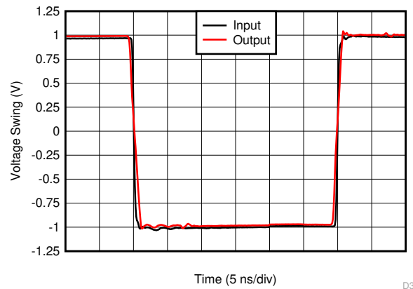
图 6-20. Large-Signal Transient Response
