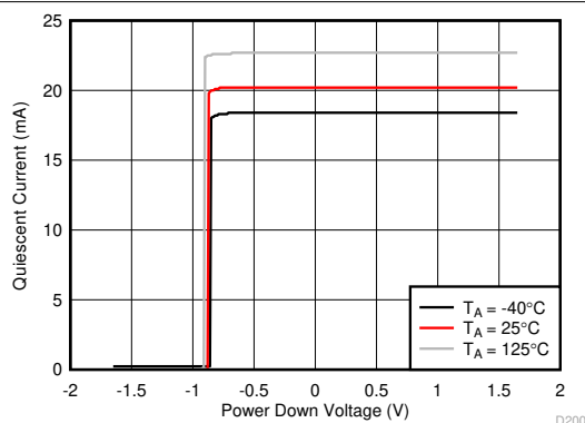
图 8-9. Switching Threshold ( \overline{\text{PD}} Pin Swept from High to Low)
