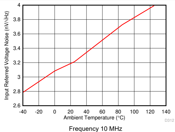
图 6-12. Voltage Noise Density vs Ambient Temperature
