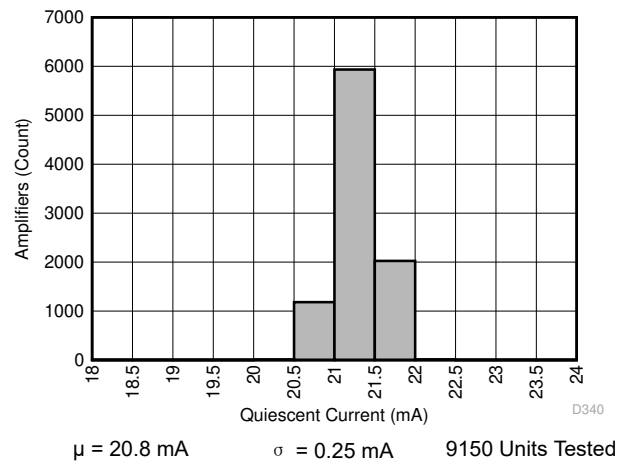
图 6-40. Quiescent Current Distribution
