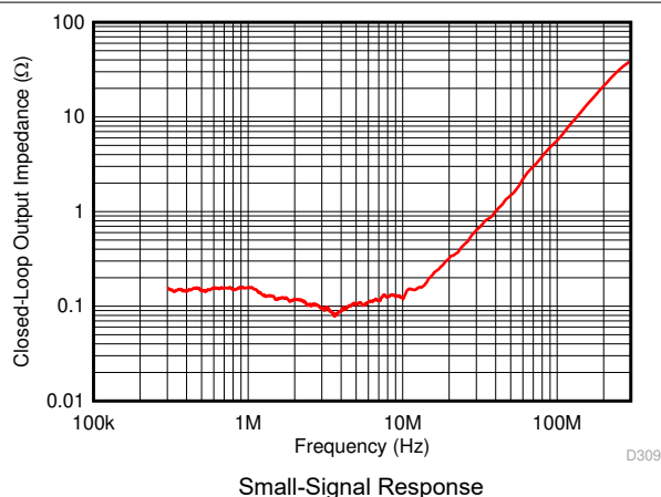
图 6-9. Closed-Loop Output Impedance vs Frequency
