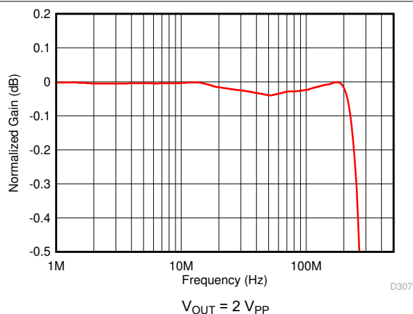
图 6-8. Large-Signal Response for 0.1-dB Gain Flatness
