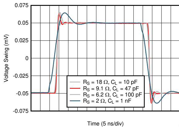
图 6-19. Small-Signal Transient Response
