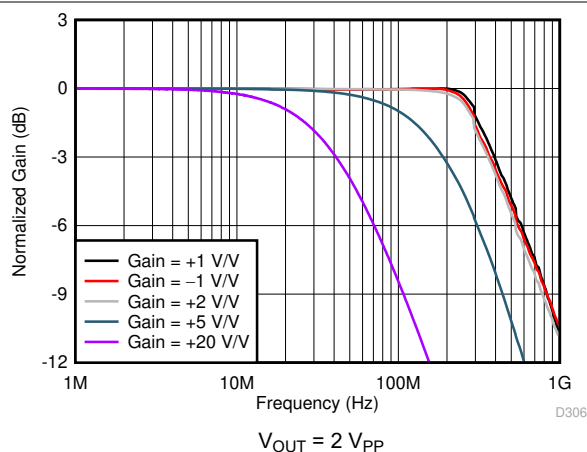
图 6-7. Large-Signal Frequency Response vs Gain
