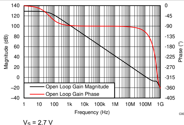
图 7-15. Open Loop Gain vs Frequency
