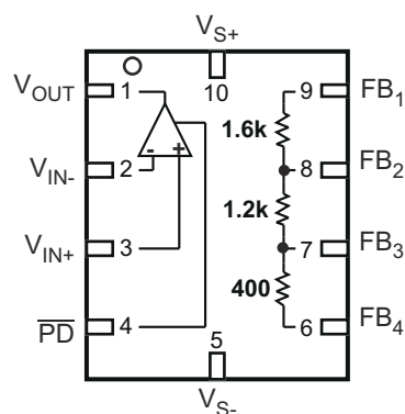
图 6-2. OPA836 RUN Package 10-Pin WQFN Top View
