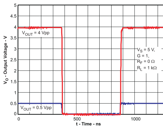
图 7-29. Noninverting Pulse Response
