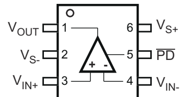
图 6-4. OPA836 DBV Package 6-Pin SOT-23 Top View
