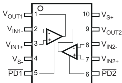
图 6-5. OPA2836 DGS Package 10-Pin VSSOP Top View
