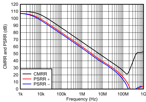
图 6-19. Common-Mode and Power-Supply Rejection Ratio vs Frequency
