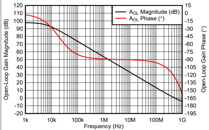
图 6-20. Open-Loop Gain Magnitude and Phase vs Frequency
