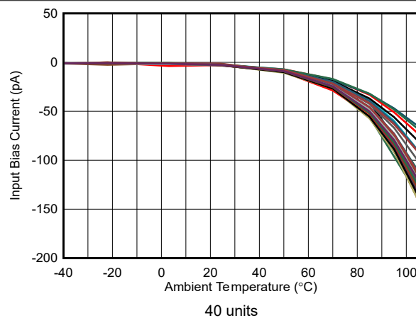
图 6-29. Input Bias Current vs Temperature
