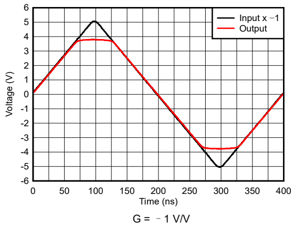
图 6-33. Inverting Output Overdrive Recovery
