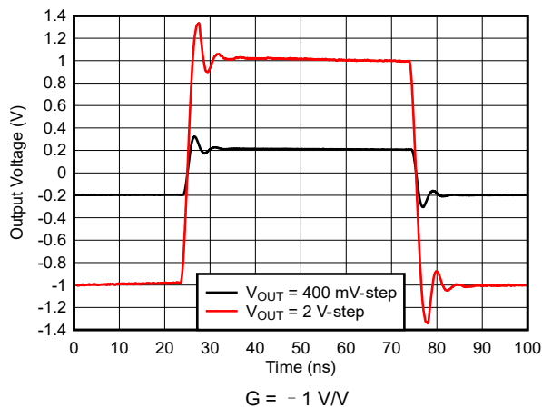
图 6-9. Inverting Large-Signal Pulse Response
