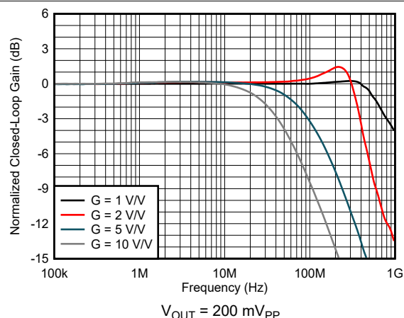
图 6-1. Noninverting Small-Signal Frequency Response
