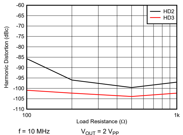
图 6-10. Harmonic Distortion vs Load Resistance
