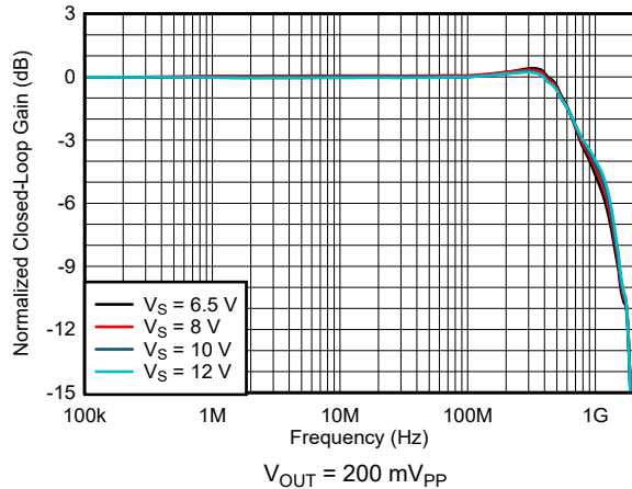
图 6-7. Noninverting Small-Signal Frequency Response Over Supply
