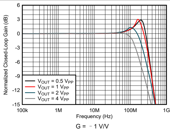
图 6-5. Inverting Large-Signal Frequency Response
