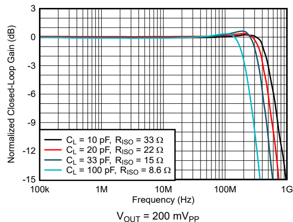
图 6-21. Frequency Response vs Capacitive Load
