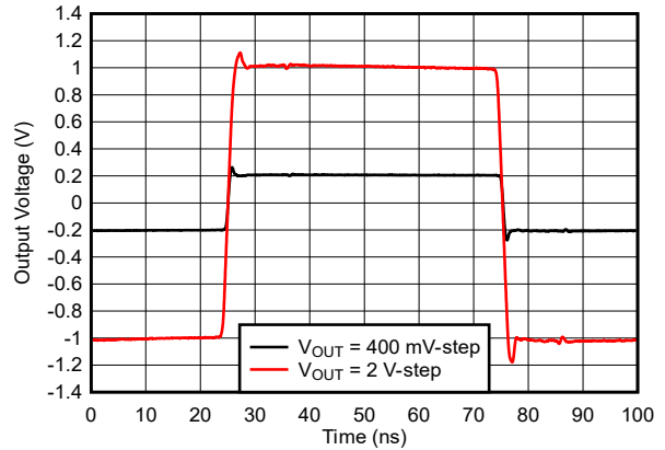
图 6-8. Noninverting Large-Signal Pulse Response
