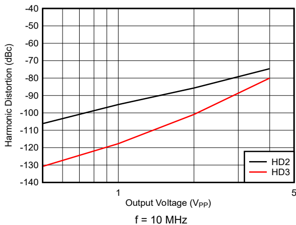
图 6-11. Harmonic Distortion vs Output Voltage
