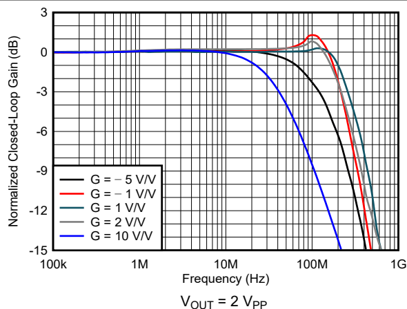
图 6-6. Large-Signal Frequency Response Over Gain
