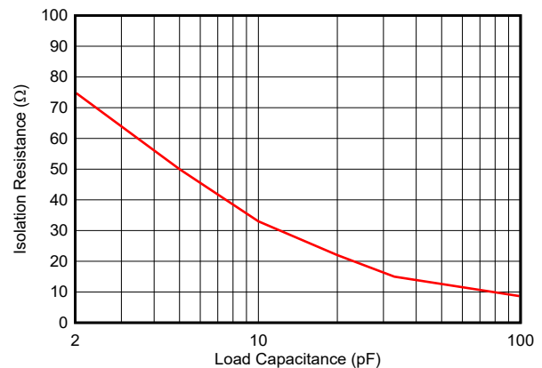
图 6-22. Recommended Isolation Resistor vs Capacitive Load
