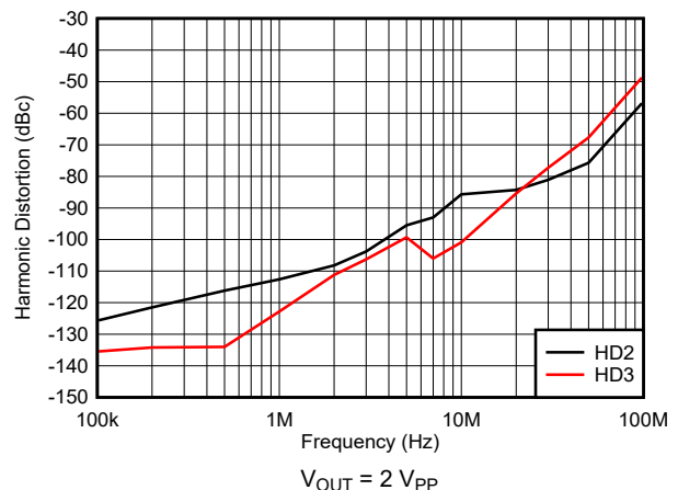
图 6-12. Harmonic Distortion vs Frequency
