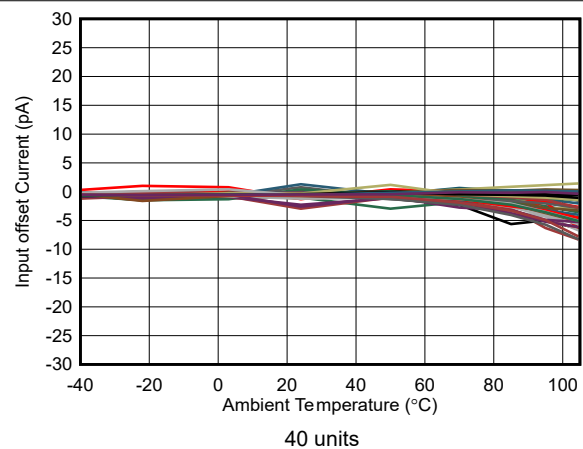
图 6-30. Input Offset Current vs Temperature
