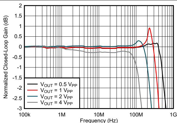
图 6-2. Inverting Small-Signal Frequency Response
