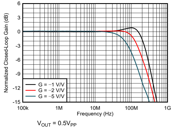
图 6-2. Inverting Small-Signal Frequency Response
