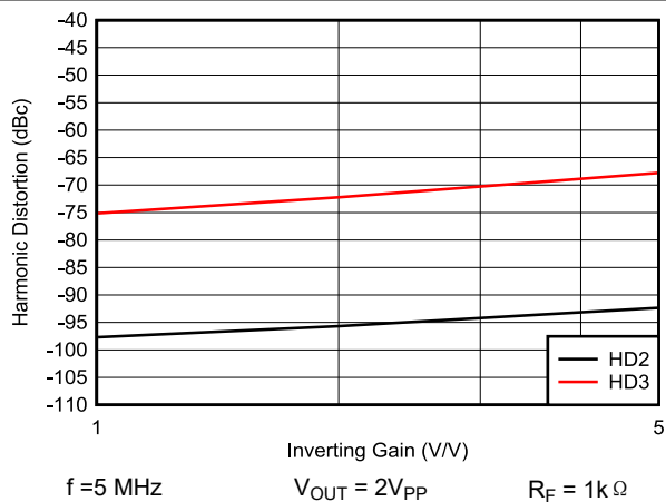
图 6-12. Harmonic Distortion vs Inverting Gain
