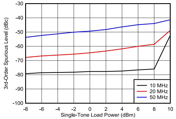
图 6-14. Intermodulation Distortion vs Load Power
