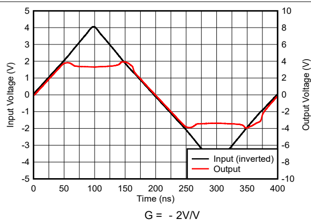
图 6-19. Inverting Output Overdrive Recovery
