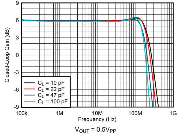
图 6-16. Frequency Response vs Capacitive Load
