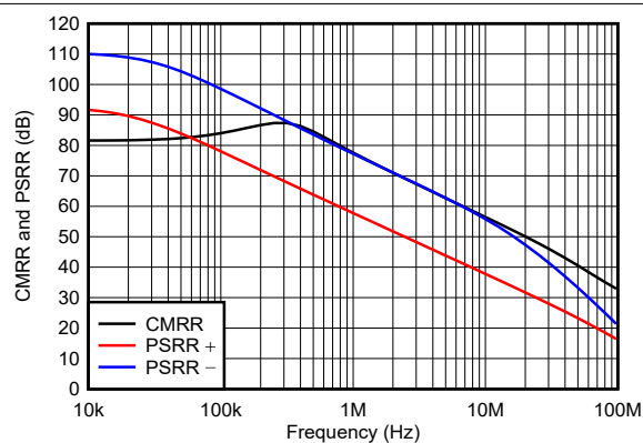
图 6-20. Common-Mode and Power-Supply Rejection Ratio vs Frequency
