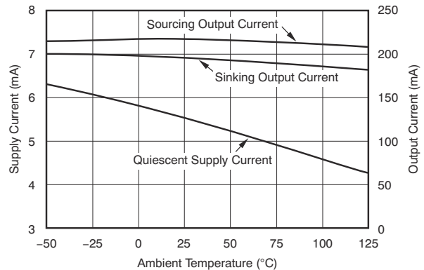
图 6-56. Typical DC Drift Over Temperature
