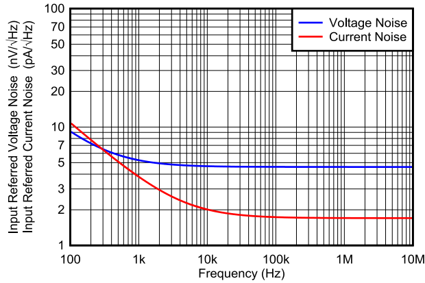
图 6-13. Voltage Noise Density vs Frequency
