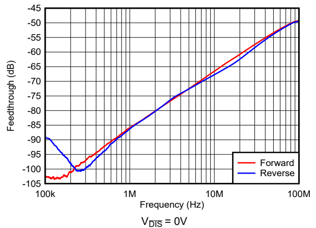
图 6-6. Disable Feedthrough vs Frequency
