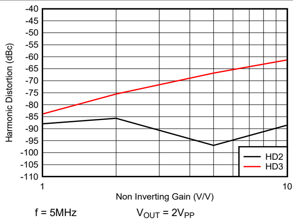
图 6-11. Harmonic Distortion vs Noninverting Gain
