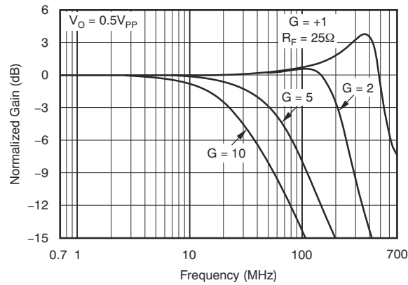
图 6-37. Small-Signal Frequency Response
