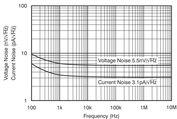
图 6-49. Input Voltage and Current Noise Density
