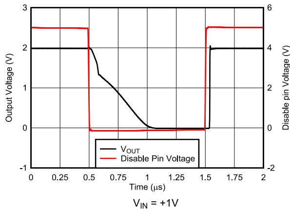
图 6-17. Enable and Disable Settling Response
