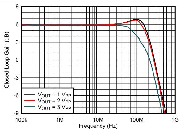
图 6-29. Noninverting Large-Signal Frequency Response
