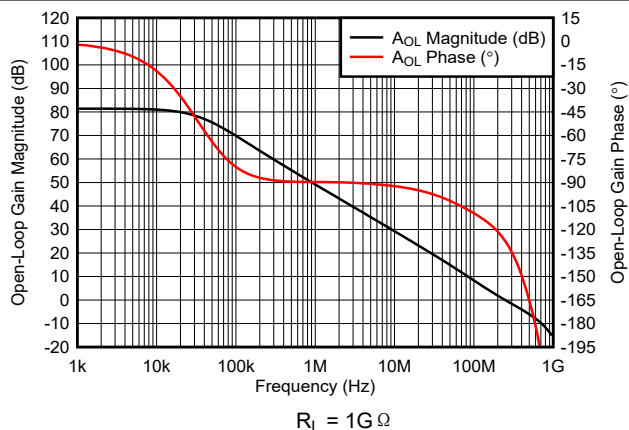
图 6-21. Open-Loop Gain Magnitude and Phase vs Frequency
