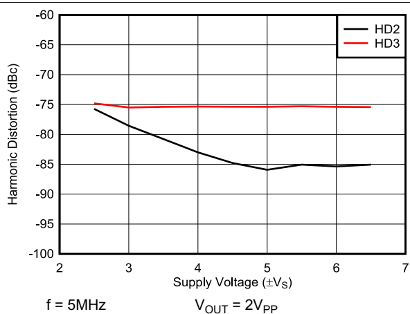
图 6-8. Harmonic Distortion vs Supply Voltage
