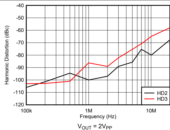
图 6-9. Harmonic Distortion vs Frequency
