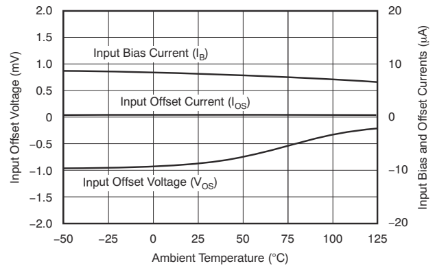
图 6-56. Typical DC Drift Over Temperature
