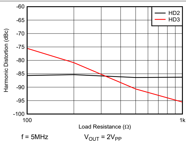
图 6-7. Harmonic Distortion vs Load Resistance
