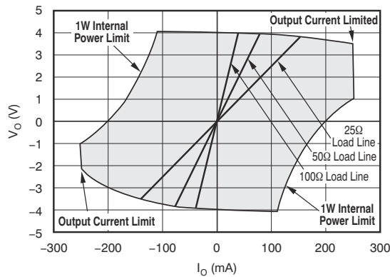
图 6-55. Output Voltage and Current Limitations
