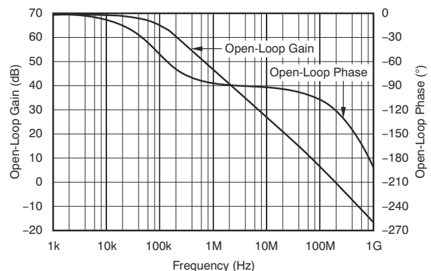
图 6-60. Open-Loop Gain and Phase
