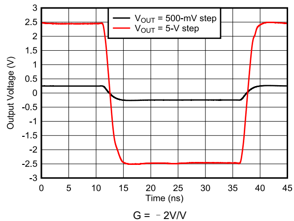
图 6-5. Inverting Pulse Response
