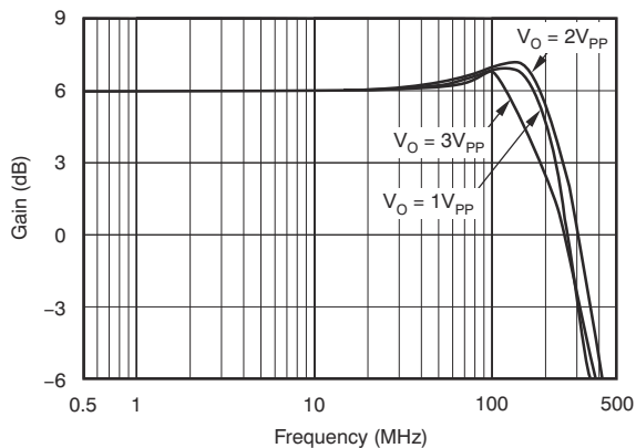
图 6-63. Large-Signal Frequency Response
