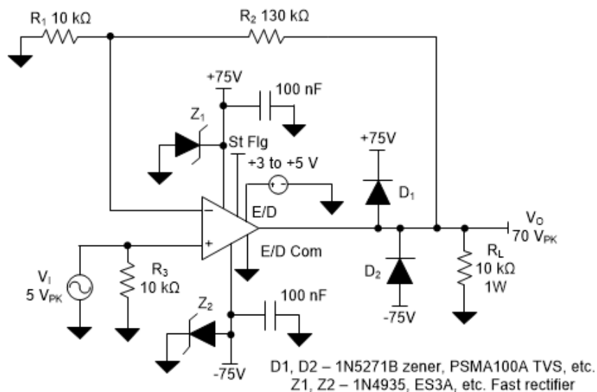
图 8-1. OPA455, High-Voltage Noninverting Amplifier, A_V = 14 V/V
