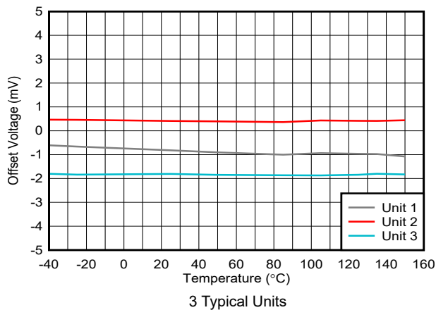
图 6-21. Offset Voltage vs Ambient Temperature
