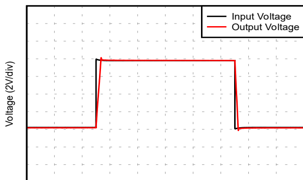
Time (20μs/div) G = +1, 4V 阶跃
