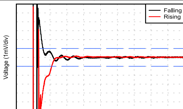
Time (10μs/div) 0.01% 趋稳 = \pm 100\mu\text{V}
