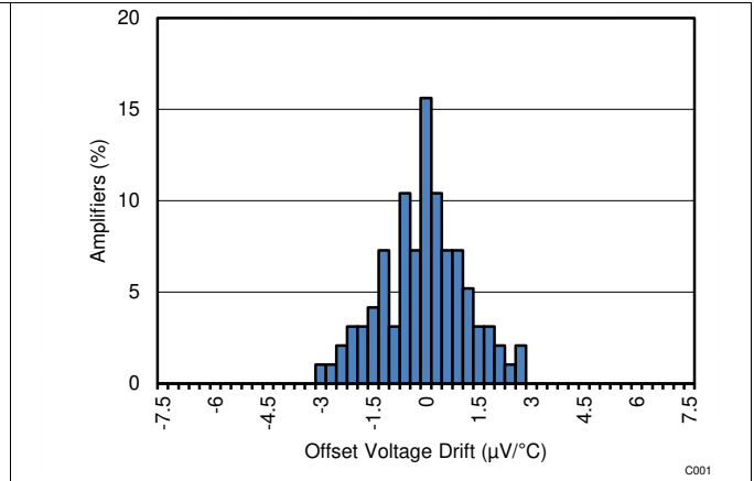
图 2. Offset Voltage Drift Distribution Histogram
