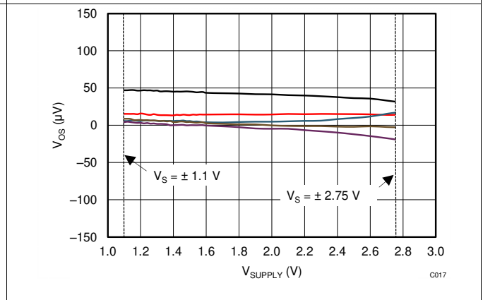
图 6. Offset Voltage vs Supply Voltage
