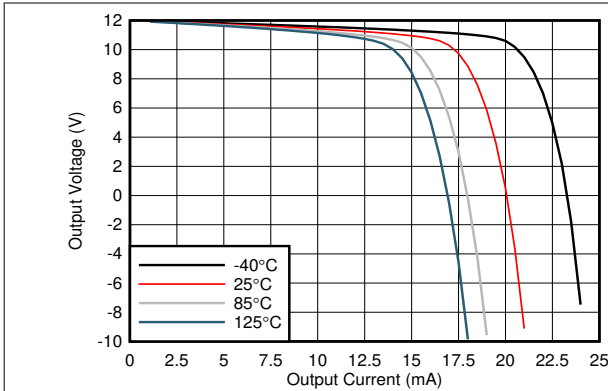
图 6-11. Output Voltage Swing vs Output Current (Sourcing)
