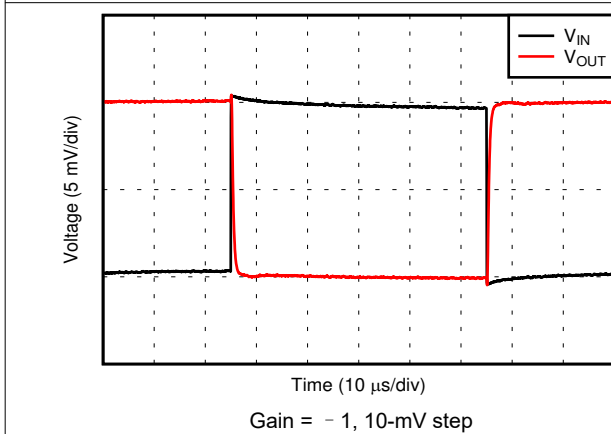
图 6-31. Small-Signal Step Response
