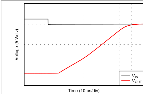
图 6-29. Negative Overload Recovery
