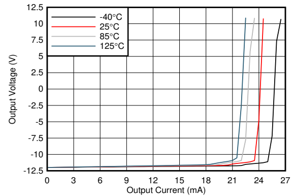
图 6-12. Output Voltage Swing vs Output Current (Sinking)
