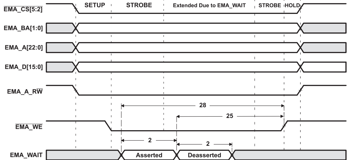
Figure 5-18. EMA_WAIT Write Timing Requirements
