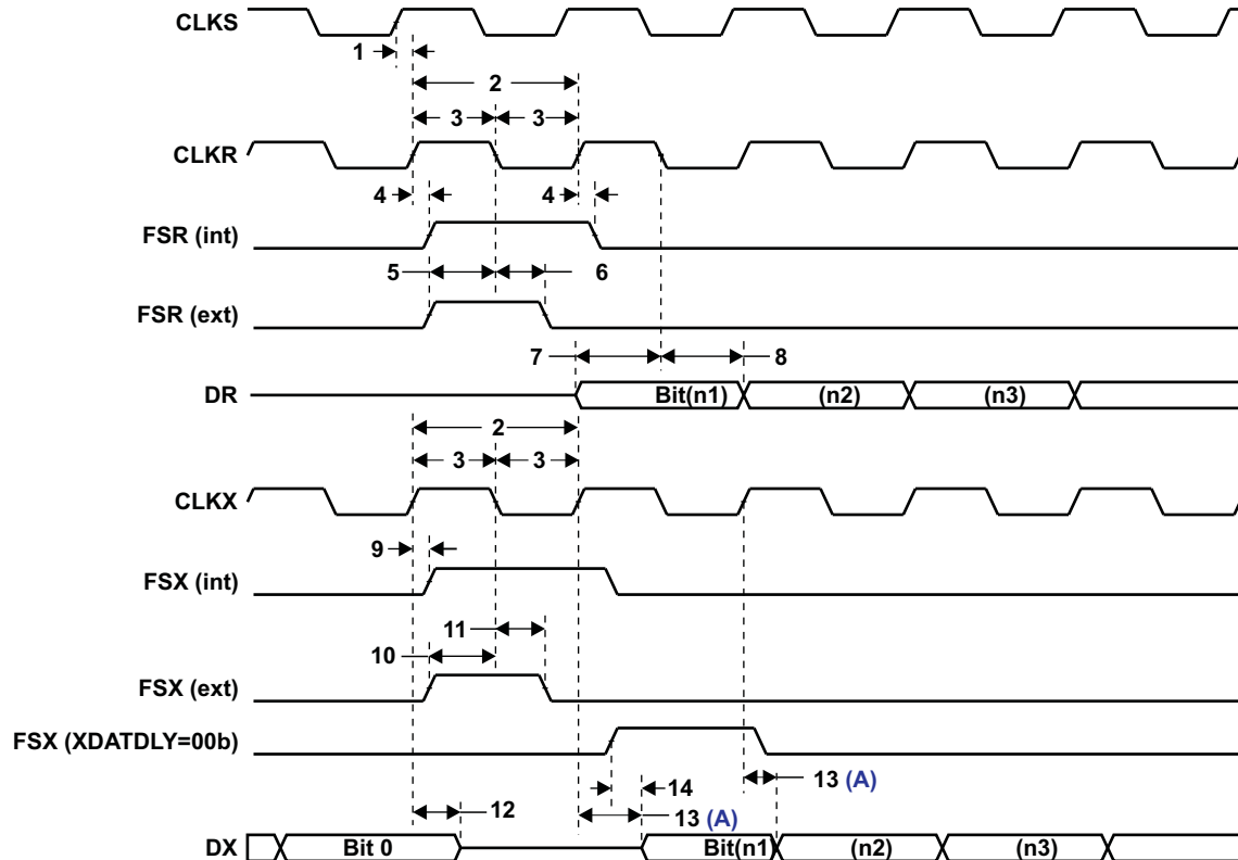
Figure 6-33. McBSP Timing
