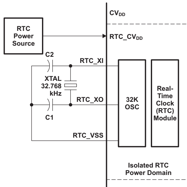
Figure 6-60. Clock Source
