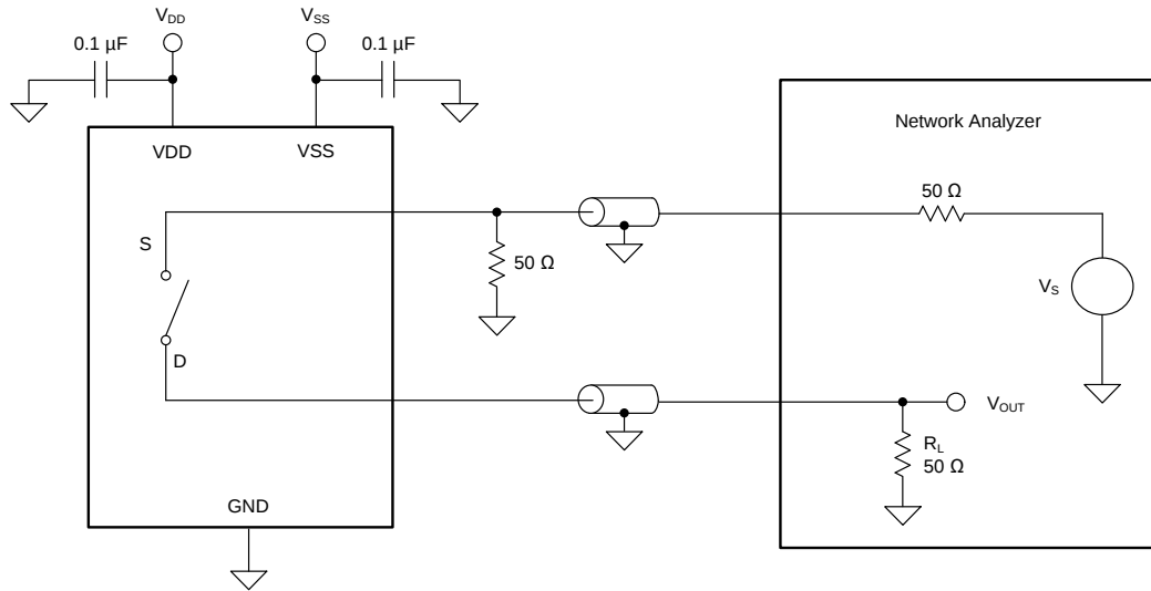
图 33. Off Isolation Measurement Setup
