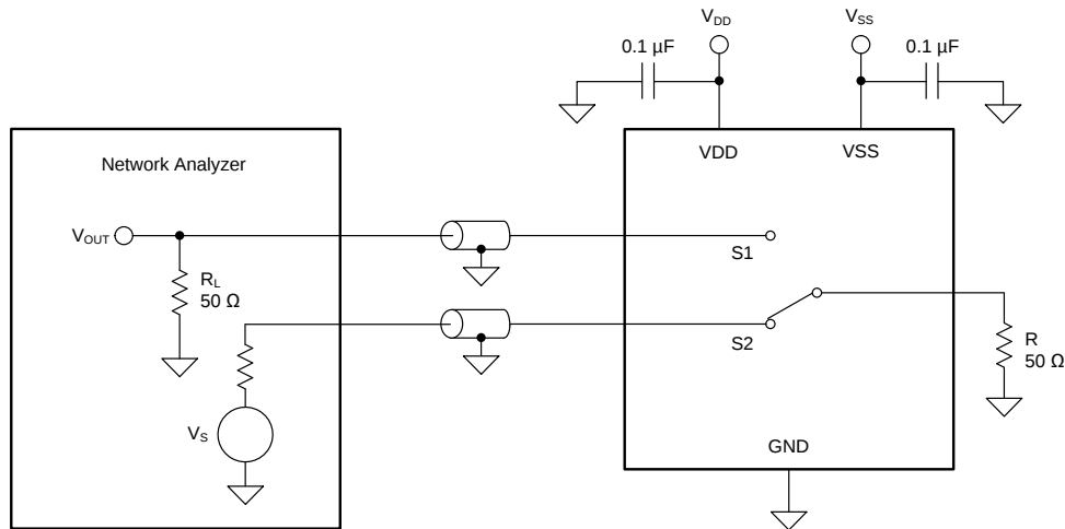
图 34. Channel-to-Channel Crosstalk Measurement Setup
