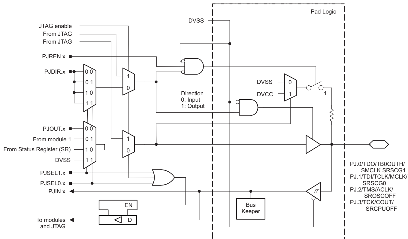
图 6-13. Port PJ (PJ.0 to PJ.3) Diagram
