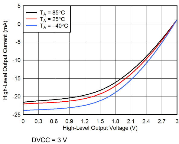
图 8-9. Typical High-Level Output Current vs High-Level Output Voltage
