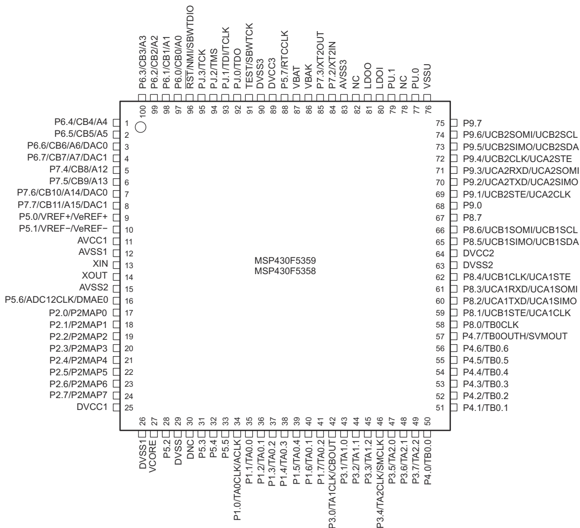
图 7-4. 100-Pin PZ Package (Top View) - MSP430F5359IPZ, MSP430F5358IPZ
