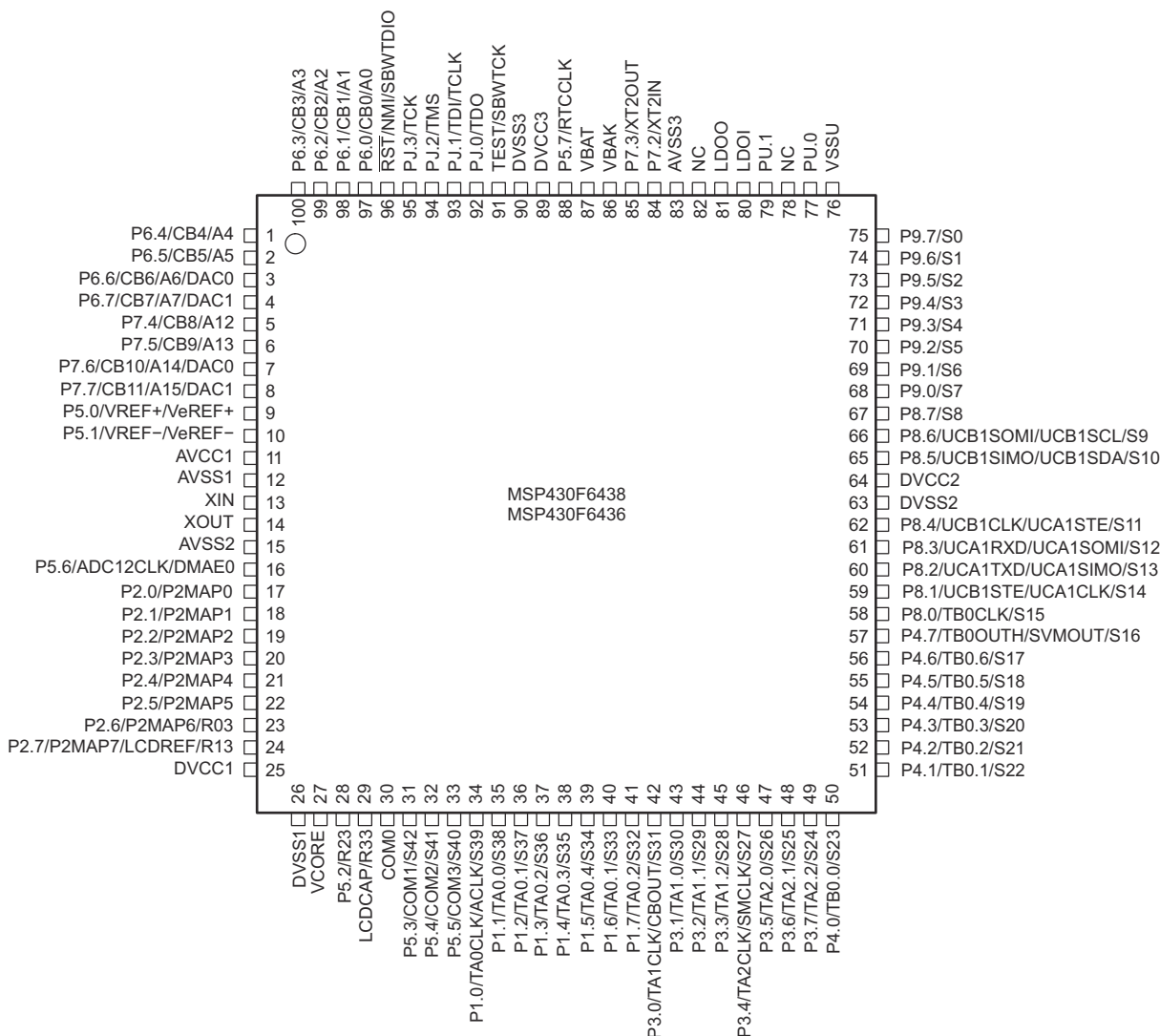
图 7-1. 100-Pin PZ Package (Top View) - MSP430F6438, MSP430F6436
