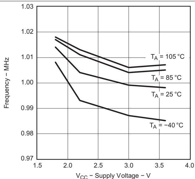
Figure 13. Calibrated 1-MHz Frequency vs Supply Voltage
