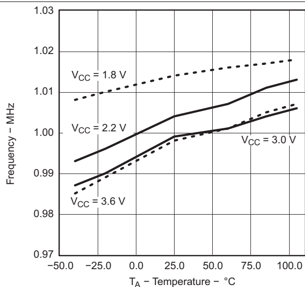
Figure 12. Calibrated 1-MHz Frequency vs Temperature
