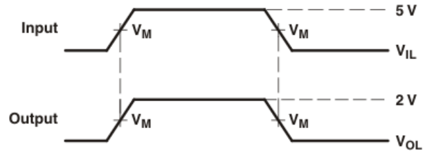
TRANSLATING DOWN
