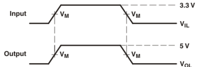
TRANSLATING UP
